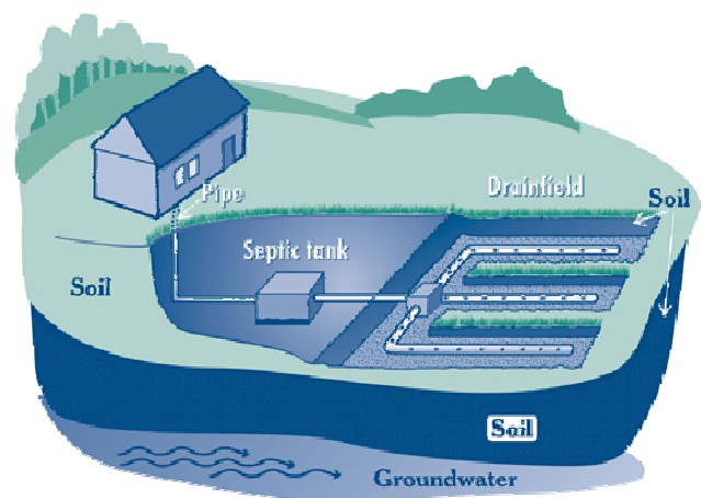
Typical onsite wastewater treatment system
